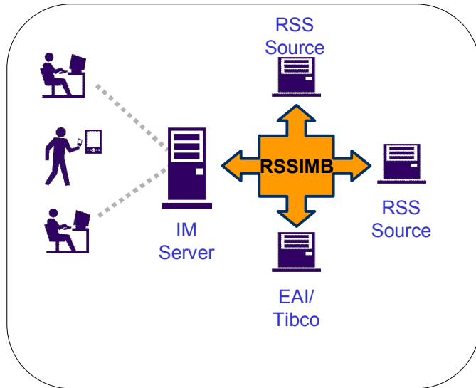
Architecture of Vayusphere's RSS to IM Bridge
